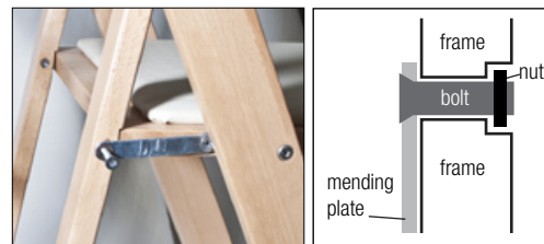
mending plate innovative bolt construction
